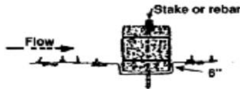
PLACEMENT DETAIL UPSTREAM ROW
