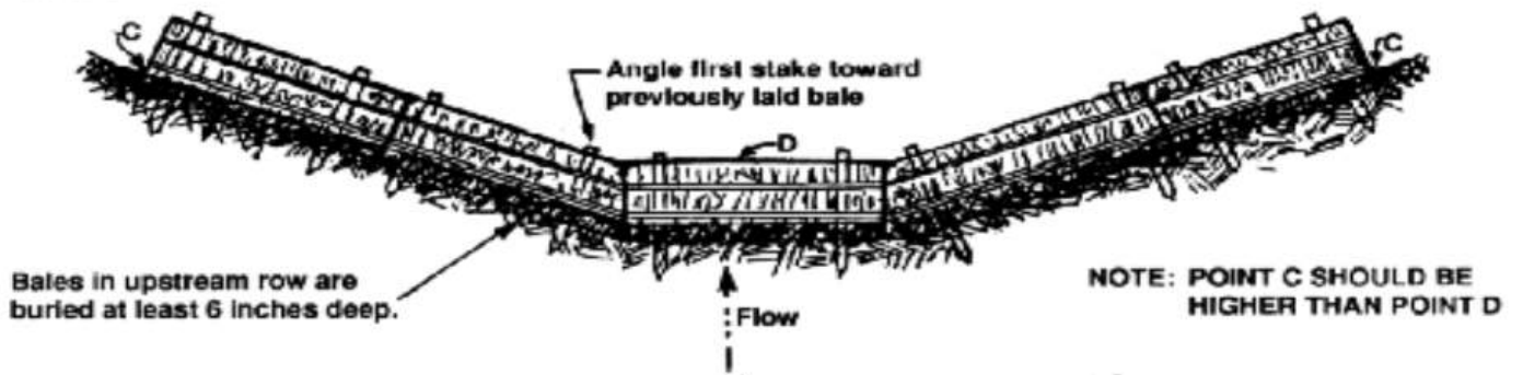
PLACEMENT DETAIL UPSTREAM ROW
